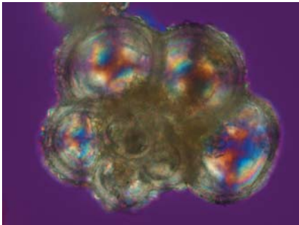
Figure 21. A juvenile Rugoglobigerina hexacamerata specimen shown in plane-polarized light (left), in crossed polars (middle top) and in crossed polars with a 530 nm compensator (middle bottom). The refractive index of the mounting medium is 1.540. An SEM image shows the same specimen (right).
