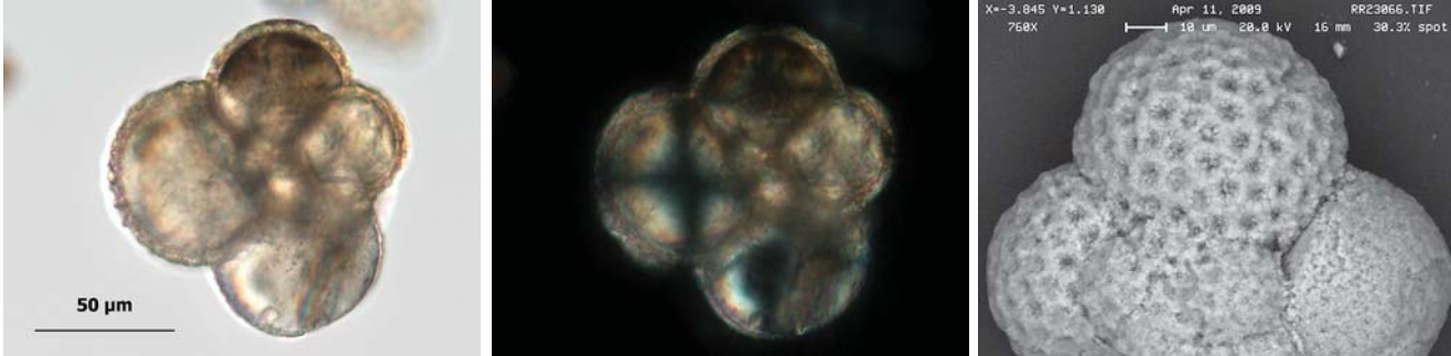
Figure 25. A Subbotina cancellata specimen shown in plane-polarized light (left), in crossed polars (middle top) and in crossed polars with a 530 nm compensator (middle bottom). The refractive index of the mounting medium is 1.540. An SEM image shows the same specimen (right).
