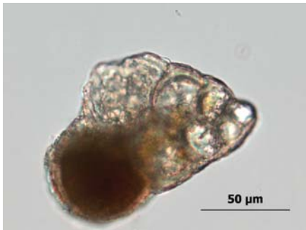
Figure 16. A Heterohelix striata specimen shown in plane-polarized light (left), in crossed polars (middle top) and in crossed polars with a 530 nm compensator (middle bottom). The refractive index of the mounting medium is 1.540. An SEM image shows the same specimen (right).
