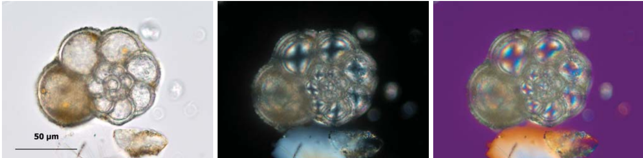
Figure 13. A foraminifer from an Alabama robbery case shown in plane-polarized light (left), in crossed polars (middle) and in crossed polars with a 530 nm compensator (right). The refractive index of the mounting medium is 1.540.
