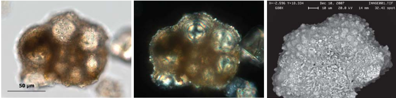
Figure 15. A Rugoglobigerina rugosa specimen shown in plane-polarized light (left), in crossed polars (middle top) and in crossed polars with a 530 nm compensator (middle bottom). The refractive index of the mounting medium is 1.540. An SEM image shows the same specimen (right).
