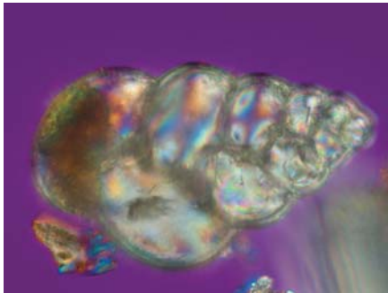
Figure 20. A Laeviheterohelix dentata specimen shown in plane-polarized light (left), in crossed polars (middle top) and in crossed polars with a 530 nm compensator (middle bottom). The refractive index of the mounting medium is 1.540. An SEM image shows the same specimen (right).
