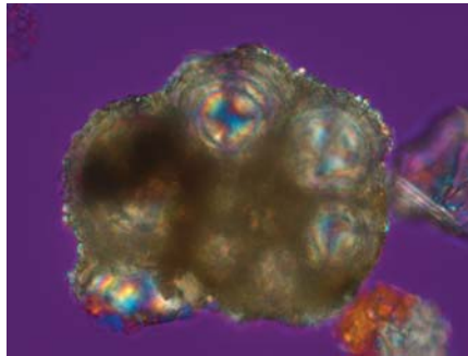
Figure 15. A Rugoglobigerina rugosa specimen shown in plane-polarized light (left), in crossed polars (middle top) and in crossed polars with a 530 nm compensator (middle bottom). The refractive index of the mounting medium is 1.540. An SEM image shows the same specimen (right).
