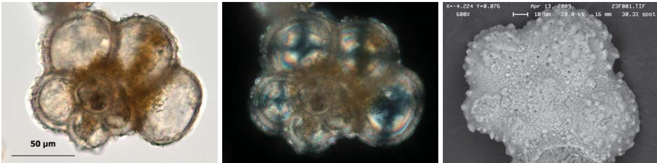
Figure 21. A juvenile Rugoglobigerina hexacamerata specimen shown in plane-polarized light (left), in crossed polars (middle top) and in crossed polars with a 530 nm compensator (middle bottom). The refractive index of the mounting medium is 1.540. An SEM image shows the same specimen (right).
