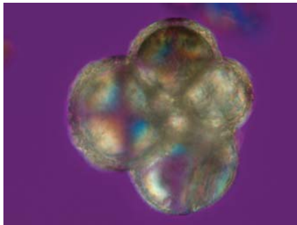
Figure 25. A Subbotina cancellata specimen shown in plane-polarized light (left), in crossed polars (middle top) and in crossed polars with a 530 nm compensator (middle bottom). The refractive index of the mounting medium is 1.540. An SEM image shows the same specimen (right).
