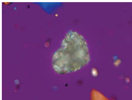
Figure 27. A small, poorly preserved foraminifer shown in plane-polarized light (left), in crossed polars (middle top) and in crossed polars with a 530 nm compensator (middle bottom). The refractive index of the mounting medium is 1.540. An SEM image shows the same specimen (right).
