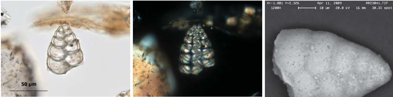
Figure 24. A Heterohelix planata specimen shown in plane-polarized light (left), in crossed polars (middle top) and in crossed polars with a 530 nm compensator (middle bottom). The refractive index of the mounting medium is 1.540. An SEM image shows the same specimen (right).
